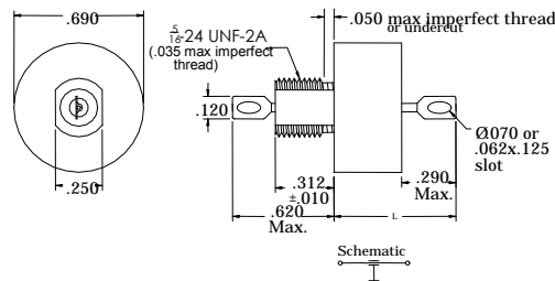
Hermetic C-Section Broadband Filter
