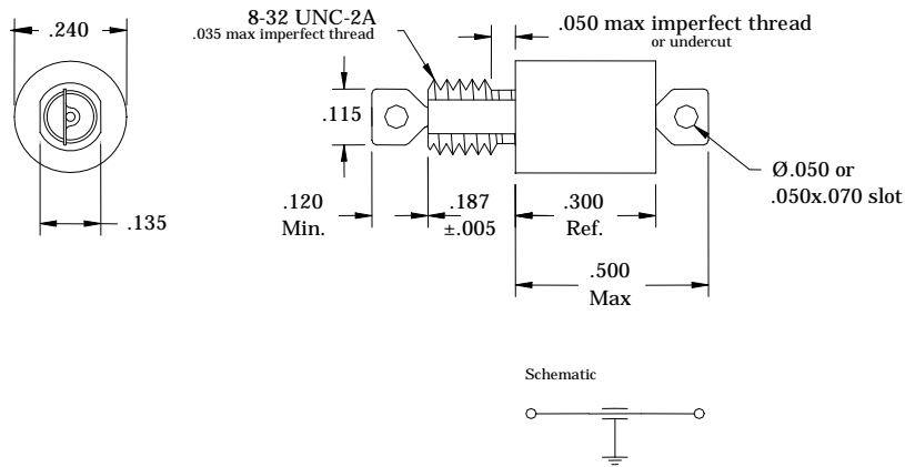
Hermetic C-Section Broadband Filter
