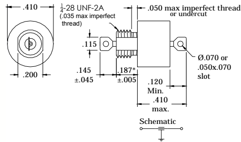
Hermetic C-Section Broadband Filter
