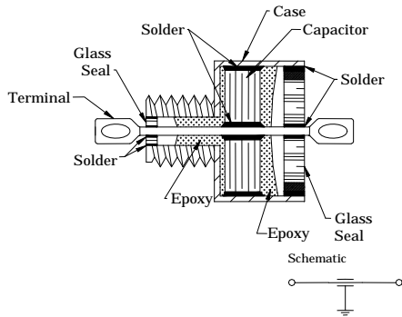
Hermetic C-Section Broadband Filter
