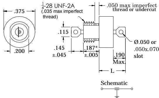
Hermetic C-Section Broadband Filter
