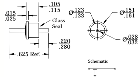
FIGURE 1 C-SECTION FILTER – SOLDER MOUNT
