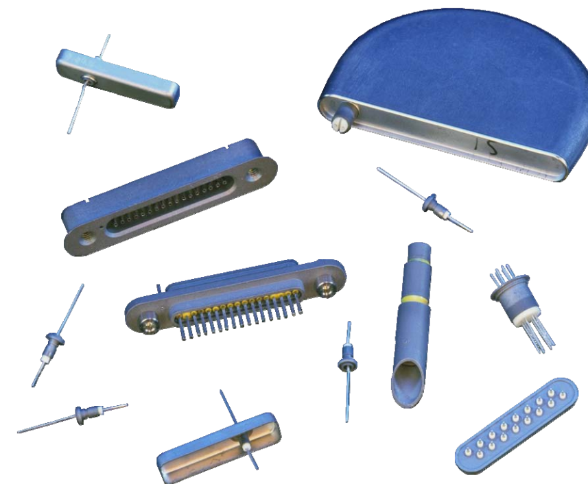
Examples of implantable packages from SOURIAU PA&E.
