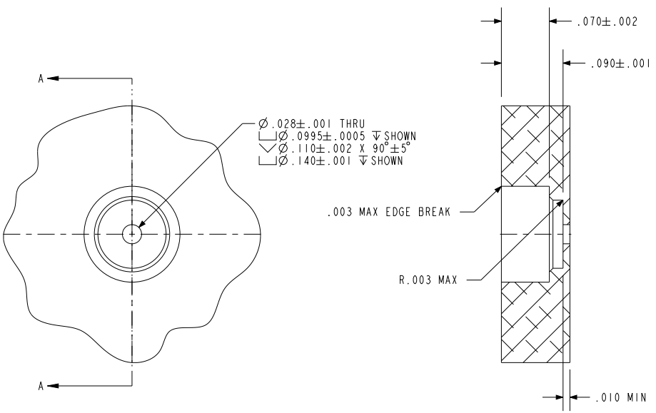
HOLE DETAIL SCALE 5.000
